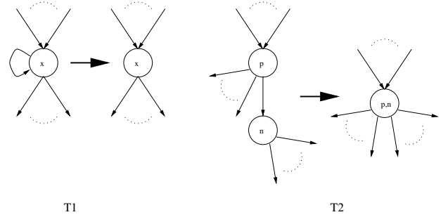
Figure 6: Graph Coalescing Transformations
